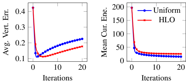
Figure 6: The average vertex errors (Avg. Vert. Err.) and total mean curvature energy (Mean Cur. Ene.) of Figure 5 with increasing iterations.
