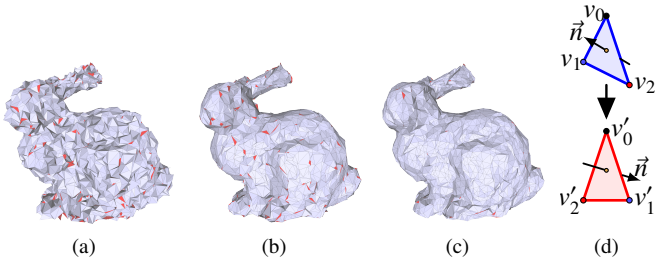
Figure 3: With and without projection. (a) Noisy bunny. (b) 1 iteration of vertex update of the half-window Laplacian without projecting onto the uniform Laplacian. (c) 1 iteration of vertex update with the half-kernel Laplacian projecting onto the uniform Laplacian. The flipped triangles are rendered in red. (d) A flipped triangle. The clock-wise or counter-clock wise order of vertices have been changed after noise contamination.
