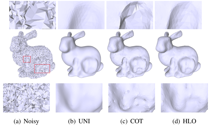
Figure 7: The comparison of smoothing results after 10 iterations on (a) a noisy bunny model ( \sigma_n = 0.8l_e ). (b) The uniform Laplacian operator. (c) The cotangent Laplacian operator. (d) The half-kernel Laplacian operator (HLO).
