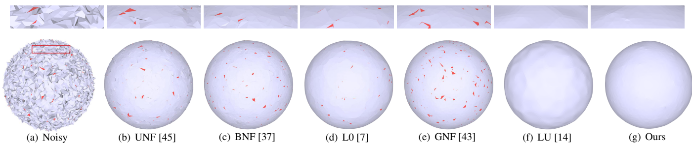
Figure 10: Sphere with heavy Gaussian noise ( \sigma_n = 0.7l_e ). The flipped triangles are rendered in red. See the close-up views for details.
