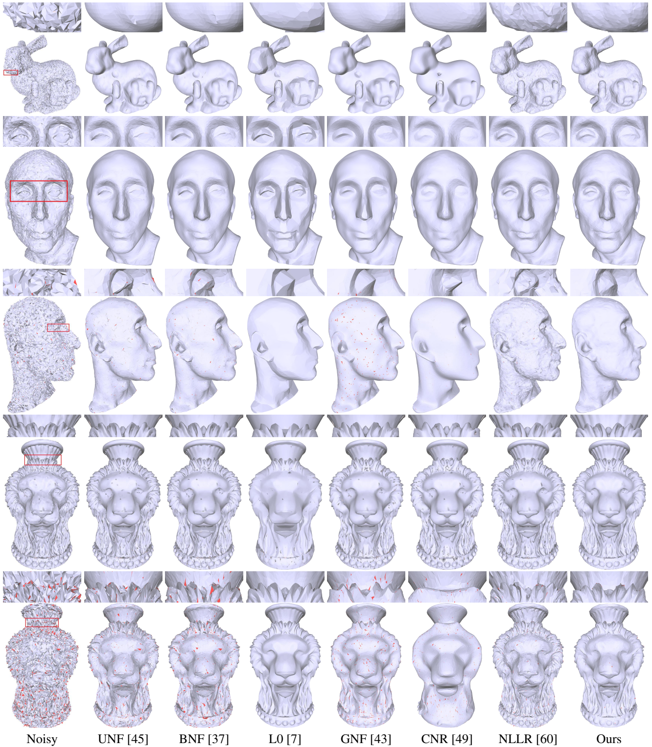
Figure 9: Models corrupted with Gaussian noise: Bunny \sigma_n = 0.5l_e , Nico \sigma_n = 0.2l_e and \sigma_n = 0.5l_e , Vase \sigma_n = 0.2l_e and \sigma_n = 0.8l_e . The flipped triangles are rendered in red.
