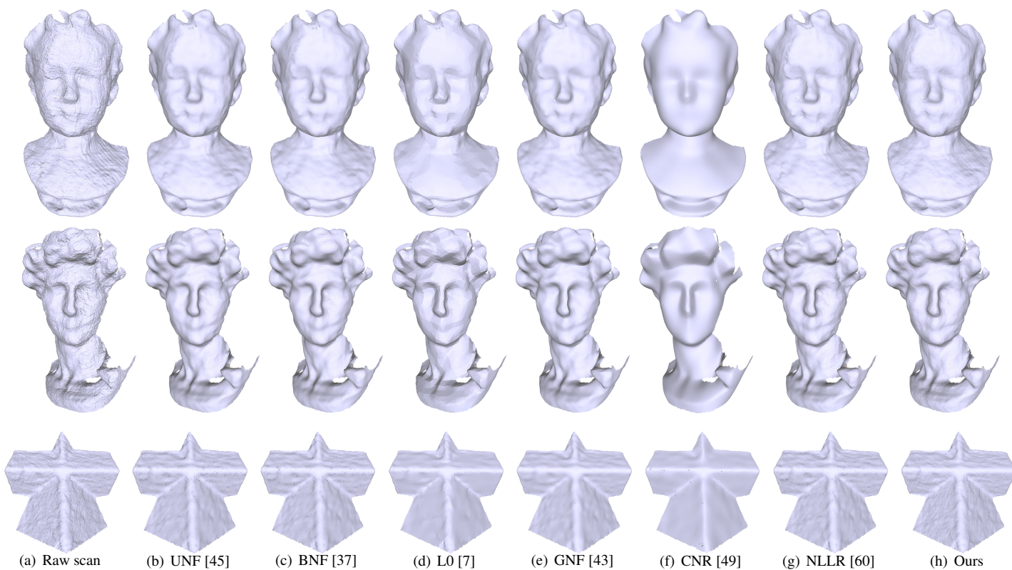
Figure 11: Results of models scanned by Microsoft Kinect.
